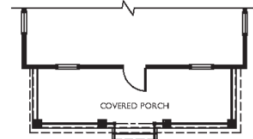
Elevation C - Covered Porch
