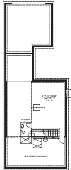
OPTIONAL FINISHED BASEMENT
