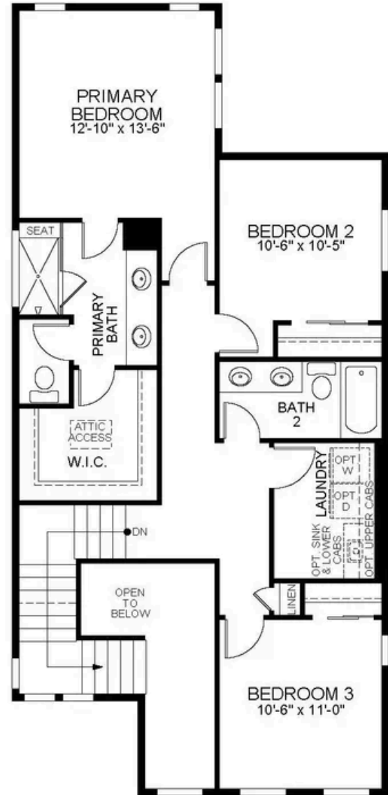
SECOND FLOOR
