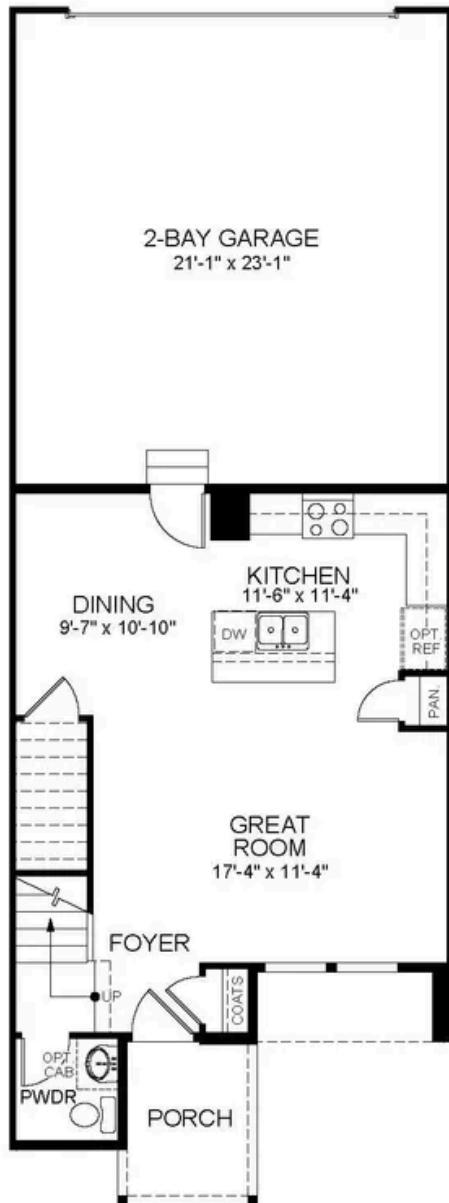
FIRST FLOOR
